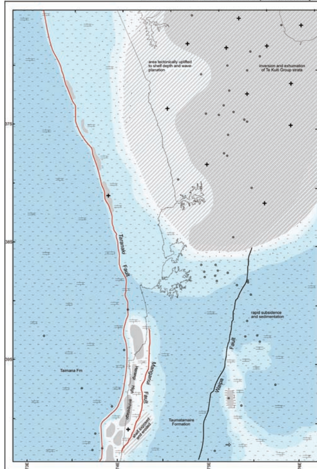
MAP (c) EARLY MIOCENE (uppermost Waitakian to lowermost Otaian) Extent of sub-Waiemata - Mahoenui Group unconformity
