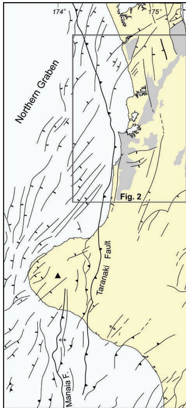
Figure 1. Location map showing structural divisions and the principal tectonic features of Taranaki Basin. Note the extent of Fig. 2.
