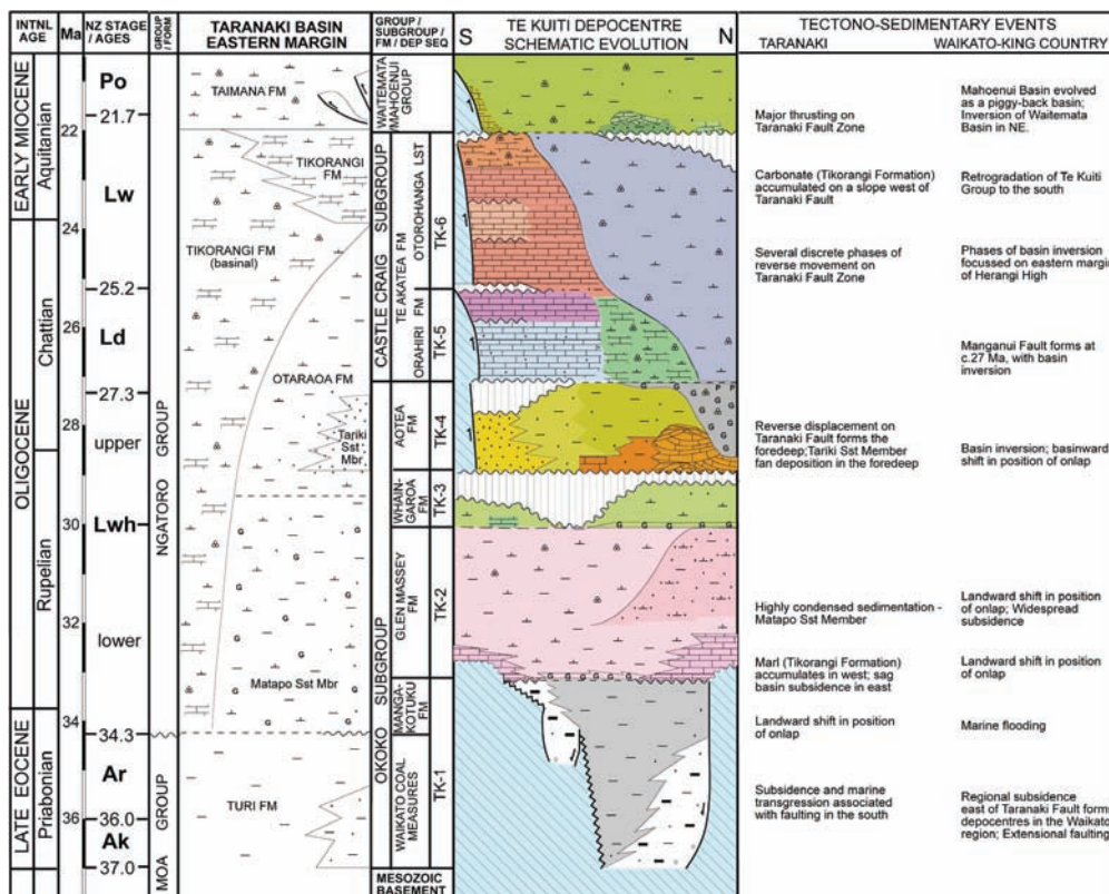
Figure 8. Chronostratigraphic panels showing comparative stratigraphy for the Taranaki Basin (from King & Thrasher, 1996) and the Te Kuiti Group, and interpretations of key tectonic events. Note that Tariki Sandstone and Hauturu Sandstone members are correlatives and their accumulation immediately postdates the transition from extension to shortening across the Taranaki Fault.
