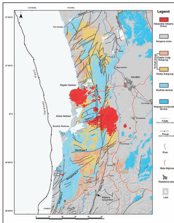
Figure 2. Geological map of the Waikato and northern part of the King Country regions, showing the distribution of the Okoko and Castle Craig subgroups of the Te Kuiti Group in relation to other units and the Taranaki Fault.
