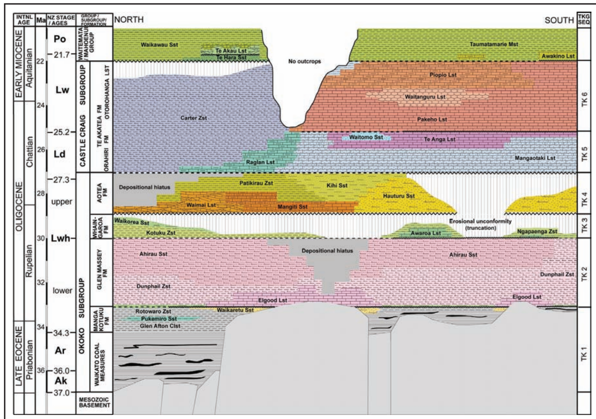
Figure 4. Chronostratigraphic panel of the Te Kuiti Group arranged north-south, showing the stratigraphic extent of unconformity-bound sequences TK1 to TK6.
