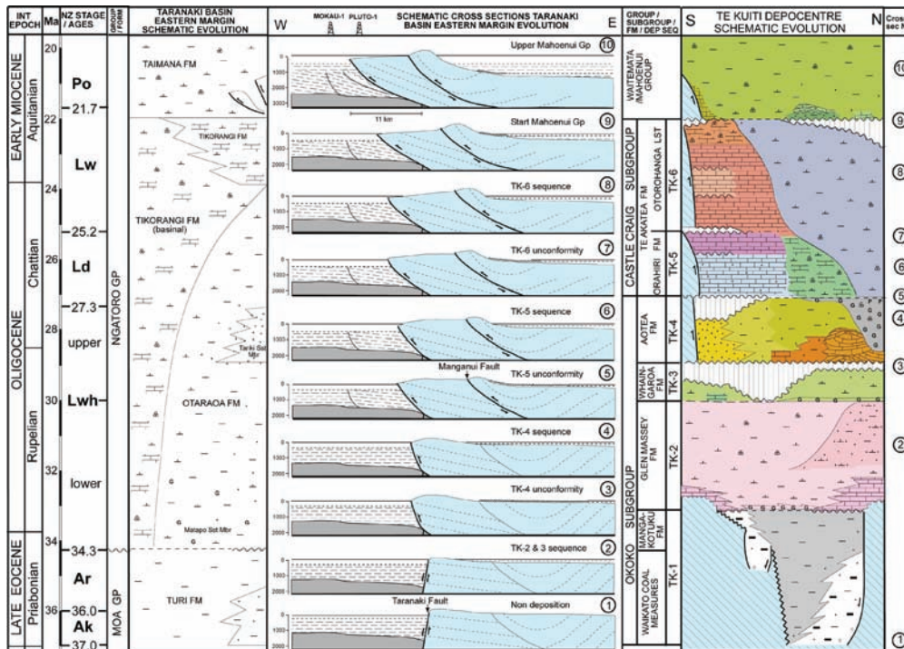
Figure 7. Schematic model to true scale of development of the Taranaki Fault Zone, constrained by its structure and the stratigraphy and basin dynamics of the Te Kuiti Group in Waikato and northern King Country depocentres. Note how a new Taranaki Fault Zone develops at c. 29 Ma, the Manganui Fault develops at c. 27 Ma, most of the displacement occurs during the Otaian, and the thrust belt is narrow (c. 15 km wide).
