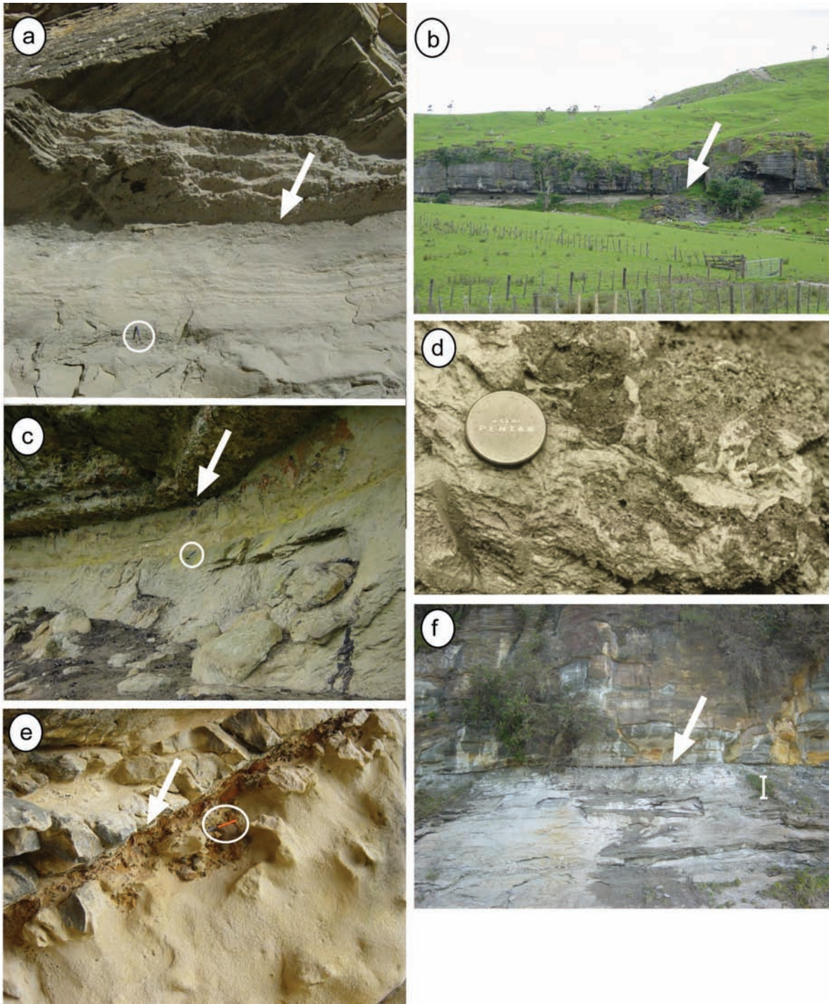
Figure 5. Examples of unconformities separating Te Kuiti Group sequences. (a) Planar contact between Kotuku Siltstone Member (TK3) and Waimai Limestone Member (TK4) at Waikawau Beach. Hammer circled for scale. (b) Sharp planar contact between Waikorea Sandstone Member (TK3) and Waimai Limestone Member (TK4), Waimai Stream Bridge, Te Akau Coast Road. (c) Planar contact between Ahirau Sandstone Member (TK2) and Hauturu Sandstone Member (TK4) at the Mahoe Road section. Hammer circled for scale. (d) Close-up view of the highly burrowed and glauconitic contact between Dunphail Siltstone Member (TK2) and overlying Hauturu Sandstone Member (TK4) at Awakino Tunnel. Photo: C.S. Nelson. (e) Scoured pebble-filled contact (arrowed) between Hauturu Sandstone Member (TK4) and Orahiri Formation (TK5) at Awakino Tunnel. Pen circled for scale. (f) Planar (arrowed) contact between Kihi Siltstone Member (TK4) and Mangaotaki Limestone Member (TK5) at the Mangaotaki Bridge section, SH3. Bar for scale is 30 cm high.
